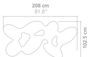
Quark 7 elements (out of edition)
