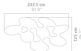
Quark 8 elements (out of edition)
