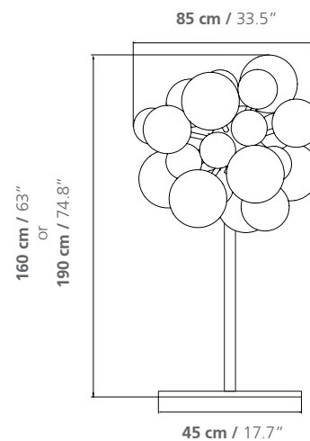
DIGIT LIGHT FULL WHITE Standing Version
