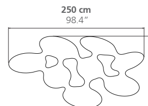
Quark 8 elements
