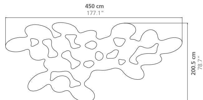
Quark 20 elements
