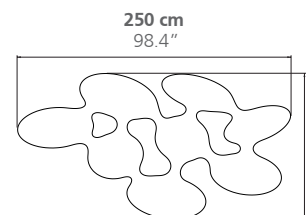
Quark 8 elements
