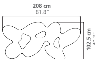
Quark 7 elements
