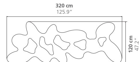
Quark 11 elements
